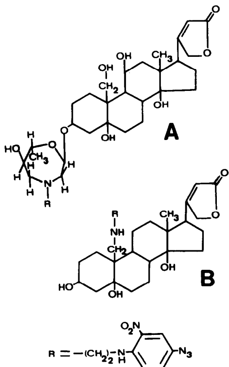
Fig.1. The structures of the photoaffinity labels. The following compounds have been used to label the (Na^+-K^+) -ATPase: (A) NAP-ouabain; (B) NAP-strophanthidin. See [2] for details.
