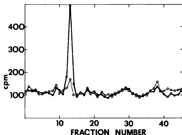
Fig.3. Photoaffinity labelling of the (\text{Na}^+ - \text{K}^+)\text{ATPase} using [^3\text{H}]\text{NAP-strophanthidin} . The enzyme was photolyzed after preincubation with 0.8 \mu\text{M} [^3\text{H}]\text{NAP-strophanthidin} (●-●) or 0.8 \mu\text{M} [^3\text{H}]\text{NAP-strophanthidin} plus 0.1 \mu\text{M} ouabain (○-○). The same SDS-gel system was used here as in fig.2.
