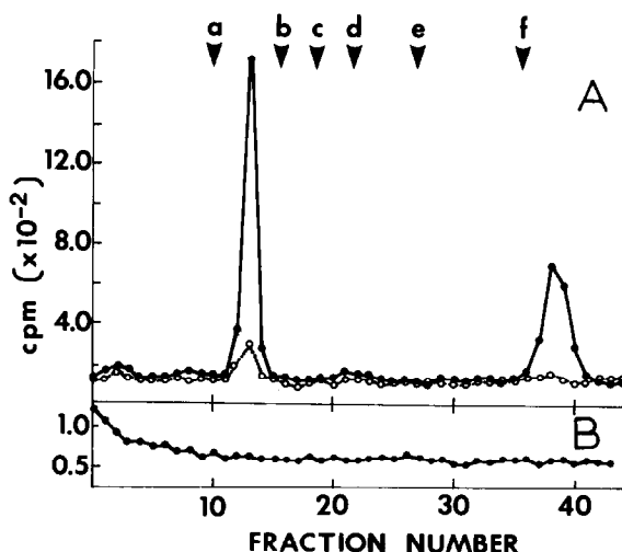
Fig.2. Photoaffinity labelling of the (Na^+-K^+) ATPase using [ ^3H ]NAP-ouabain. Panel A shows the pattern of radio-labelling after photolysis when the proteins are separated by SDS—gel electrophoresis with an acrylamide gradient of 10–30% (w/v). The experimental details are in the text. The enzyme was photolyzed after incubation with 0.8 \mu M [ ^3H ]NAP-ouabain (●—●) or with 0.8 \mu M [ ^3H ]NAP-ouabain plus 0.1 mM ouabain (○—○). The gels were calibrated using molecular weight standards prepared according to [7]. The labelled arrows indicate the mobility of the following molecular weights: (a) 132 000; (b) 66 000; (c) 57 200; (d) 42 900; (e) 28 600; (f) 14 300. Panel B shows the radioactivity pattern for photolyzed [ ^3H ]NAP-ouabain when it is applied directly to the gel.
